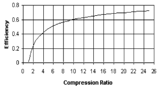
Theoretical Efficiency - Air Cycle
